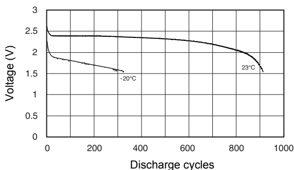
Discharge Characteristics 900mA, 3 seconds on / 27 seconds off
