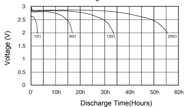
Continuous Discharge at 23°C
